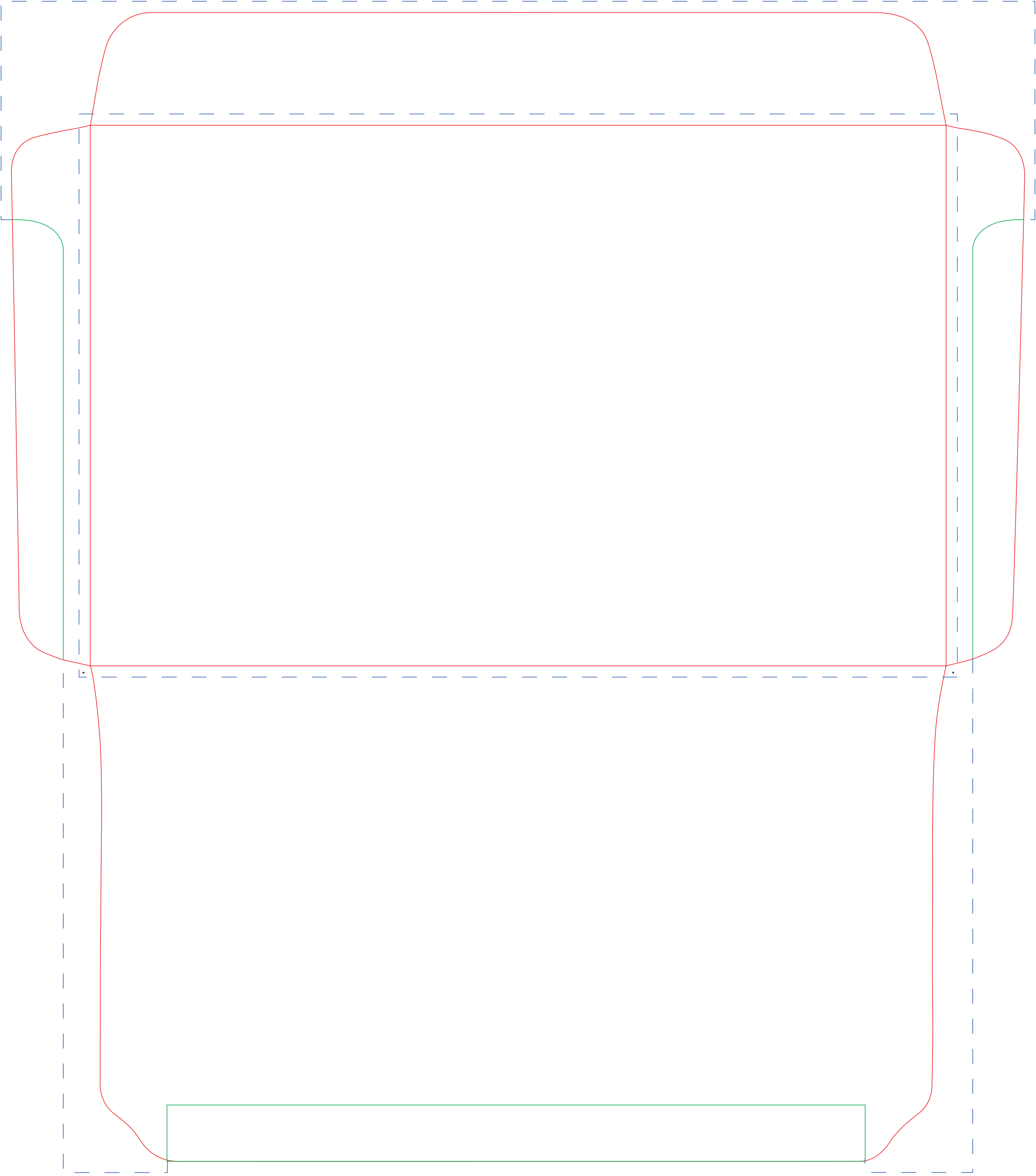
CROWN ENVELOPE 6 X 9-1/2 Booklet With 1-1/4" Seal Flap Layered Template
